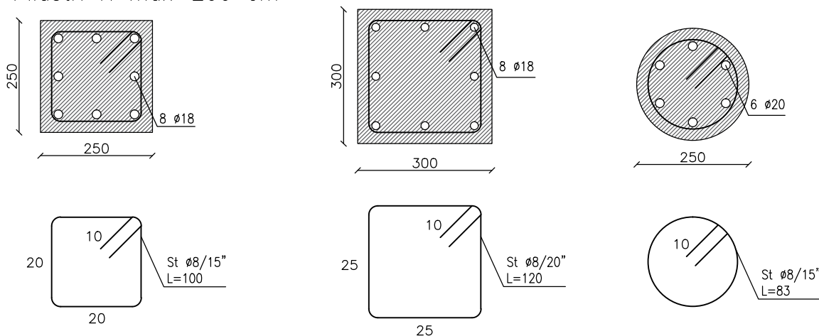
Pilastri H max=200 cm
